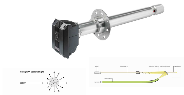
PCME QAL 181 ProScatter™ instrument
