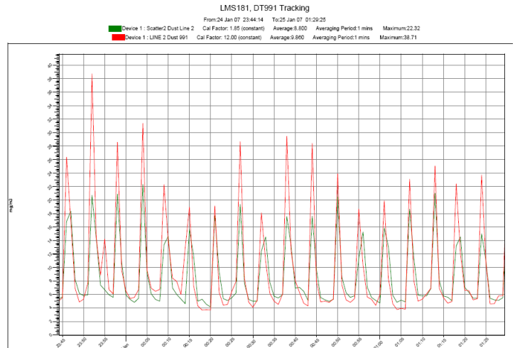
PCME QAL 181 and PCME QAL 991 tracking bag pulsing
