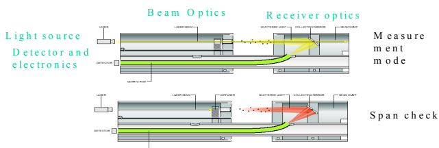
Diffuser creates scatter in span check
