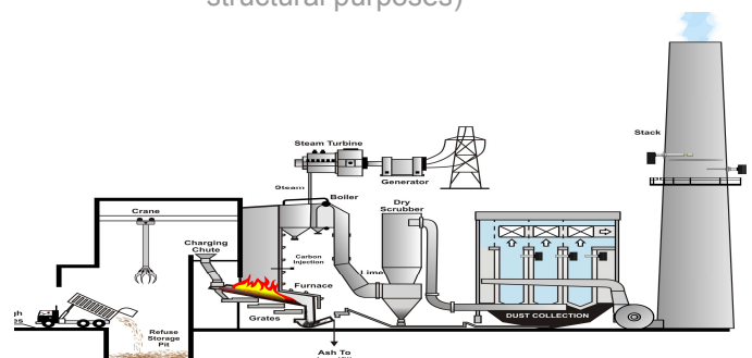
Schematic of pollution abatement equipment
